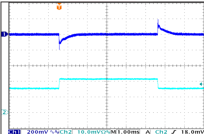
Figure 11: Output Voltage Response to Step-Change in Load Current , (50%-75%-50% of I_{out(max)} ; dI/dt = 1 A/\mu s ). Load cap: 1 µF ceramic and 100 µF electrolytic capacitors. Ch 1: Vout (200 mV/div); Ch 2: Iout (20 A/div). Timescale: 1.00ms/div.
